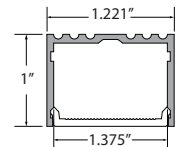
ALTN-CHAN-SLV-6.5 Anodized Aluminum Extrusion, available in 6.5' lengths
